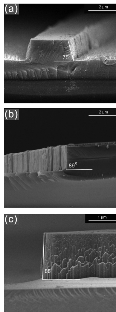
FIG. 5. SEM images of etched LiNbO 3 cross section with RIE power at (a) 60 W, (b) 90 W, and (c) 150 W. Slope angles are shown.
